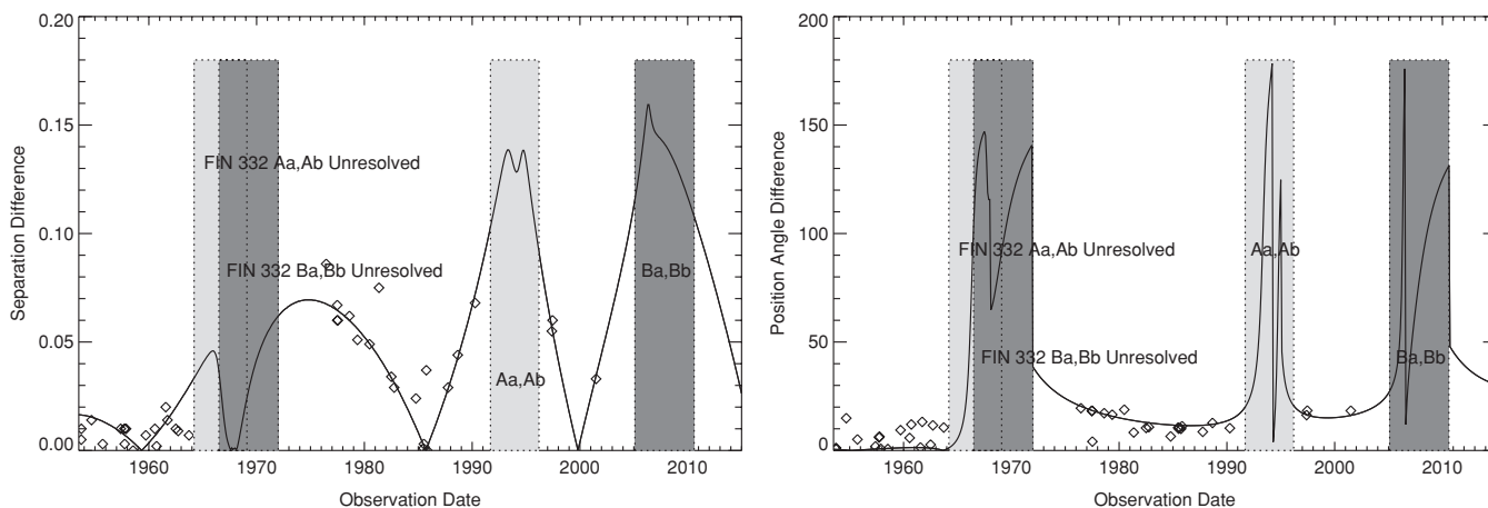
Figure 2. Difference in separation and P.A. between FIN 332 Aa, Ab and Ba, Bb. The solid curve indicates the predicted difference based on the orbits of Section 5.1. The diamonds represent the differences between measures of Aa, Ab and Ba, Bb when they were made at the same time by the same observer. The lighter shaded areas from 1964.2 to 1969.1 and 1991.7 to 1996.2 are dates when Aa, Ab is predicted to be closer than 0''.05 . The darker shaded areas from 1966.5 to 1972.0 and 2005.1 to 2010.6 indicate the range of dates when the orbit predicts Ba, Bb to be closer than 0''.05 .
