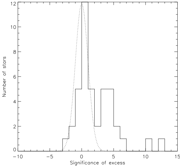
Fig. 3. Histogram of the excess significance ( \chi_f = f_{CSE}/\sigma_f ) in our sample, compared to a centred Gaussian distribution (dotted line).
