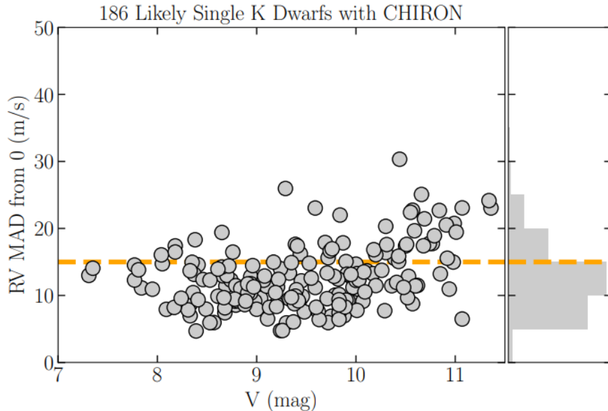
Figure 2: RV MAD (Mean Absolute Deviation) vs. V-magnitude
