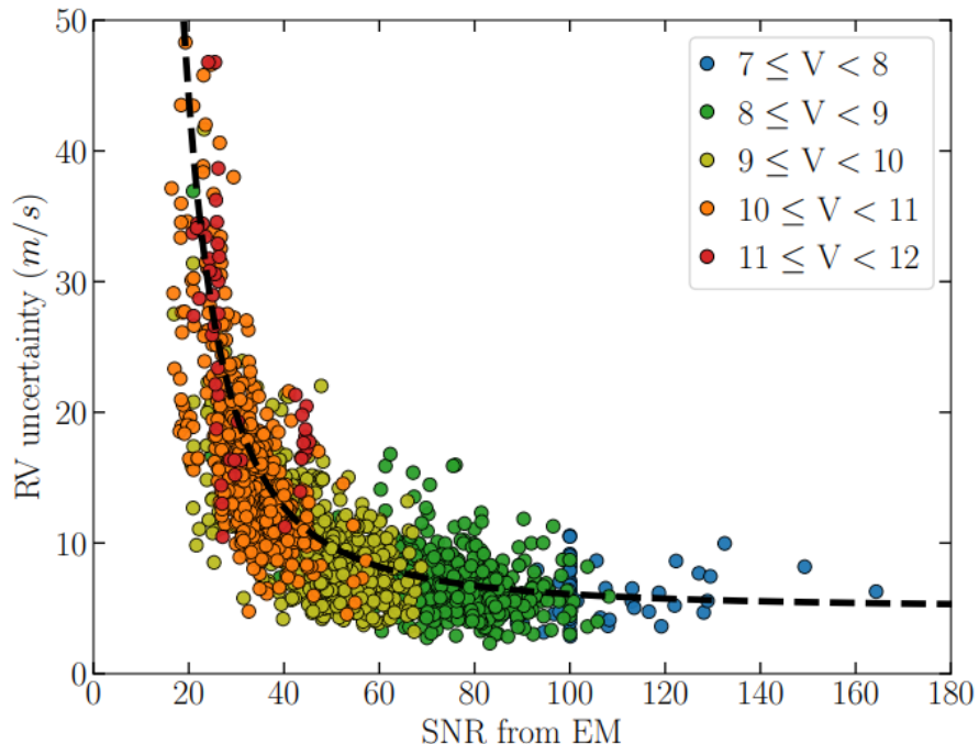
Figure 1: SNR calculated from CHIRON's exposure meter (EM) versus RV uncertainty for individual spectra of K dwarfs, color-coded by stellar V magnitude. Each of the 1784 data points represents a single spectrum. The dashed line is described by Equation (1) and is derived using observations with exposure times of 900 sec. The slight overabundance of points at SNR = 100 is the result of observations that were stopped before 900 sec, when SNR reached 100.
